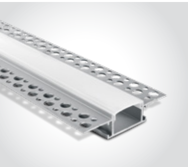
7904TR/AL | 2m Trimless profile + PC opal diffuser | Aluminium Suitable for 7820, 7829, 7829A, 7835, 7839, 7844, 7844E, 7846 & 7875 LED Strips 20mm
