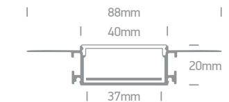
7904ATR/AL | 2m Trimless profile + PC opal diffuser | Aluminium Suitable for 7820, 7829, 7829A, 7835, 7839, 7844, 7844E, 7845, 7846, 7875 & 7887 LED Strips 20mm
