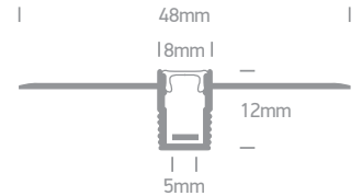
7901TR/AL | 2m Trimless profile + PC opal diffuser | Aluminium Suitable for 7820, 7823, 7829, 7829A, 7839, 7843, 7843E, 7844 & 7844E LED Strips 10mm
