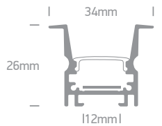
7903TR/W | 2m Trimless profile + PC opal diffuser | Aluminium | Suitable for 7820, 7829, 7829A, 7839 & 7843 LED Strips 12mm
