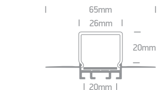
7904ATR/AL | 2m Trimless profile + PC opal diffuser | Aluminium Suitable for 7820, 7829, 7829A, 7835, 7839, 7844, 7844E, 7845, 7846, 7875 & 7887 LED Strips 20mm
