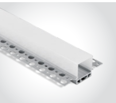
7904ATR/AL | 2m Trimless profile + PC opal diffuser | Aluminium Suitable for 7820, 7829, 7829A, 7835, 7839, 7844, 7844E, 7845, 7846, 7875 & 7887 LED Strips 20mm
