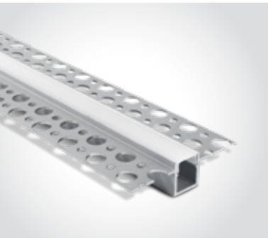
7901TR/AL | 2m Trimless profile + PC opal diffuser | Aluminium Suitable for 7820, 7823, 7829, 7829A, 7839, 7843, 7843E, 7844 & 7844E LED Strips 10mm
