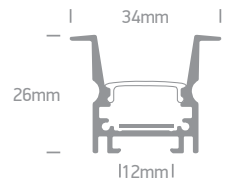
7903R/B | 2m Recessed profile + PC opal diffuser | Aluminium | Suitable for 7820, 7829, 7829A, 7839 & 7843 LED Strips 12mm
