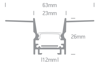
7903TR/B | 2m Trimless profile + PC opal diffuser | Aluminium | Suitable for 7820, 7829, 7829A, 7839 & 7843 LED Strips 12mm
