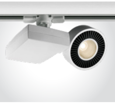
65620TA | 15W | COB LED | Die cast
