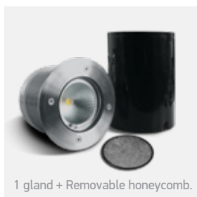
69050 | 20W | COB LED | Dimmable | Stainless steel 316 + tempered glass
