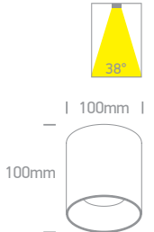
Optional Brass reflector code 050106C/BS.
